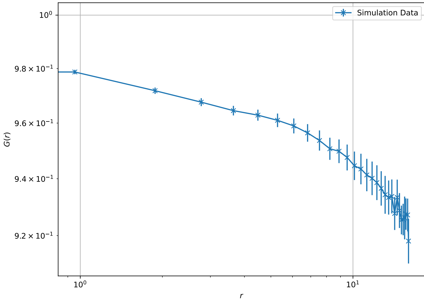
Correlation Function at T = 1.00e - 01 , L = 16 (Log-Log Scale)
