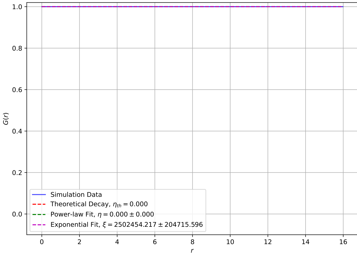
Correlation Function at T = 1.00\text{e} - 05 , L = 16
