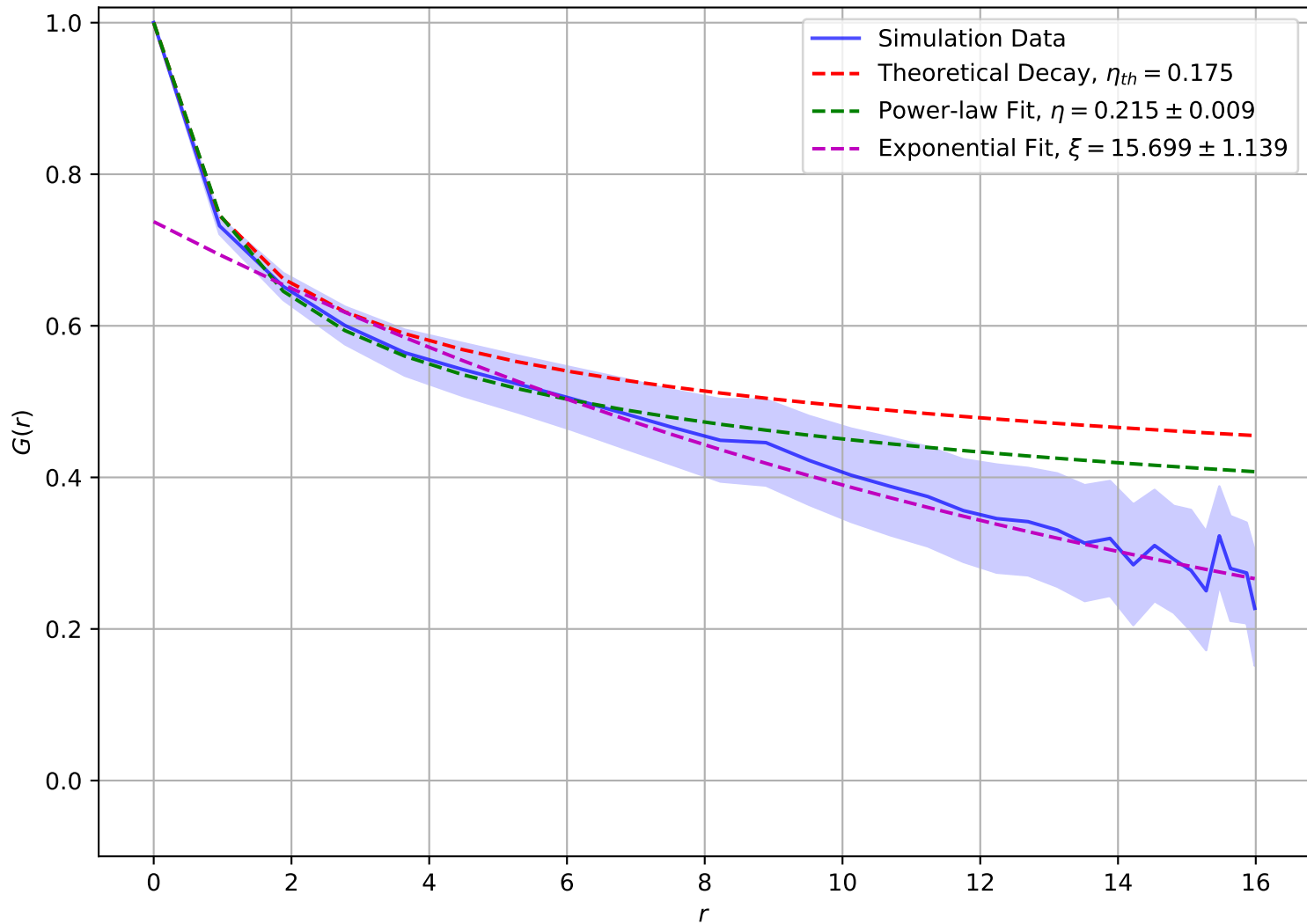
Correlation Function at T = 1.10e + 00 , L = 16
