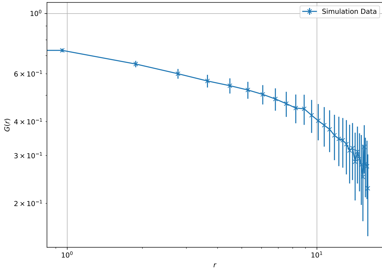
Correlation Function at T = 1.10e + 00 , L = 16 (Log-Log Scale)
