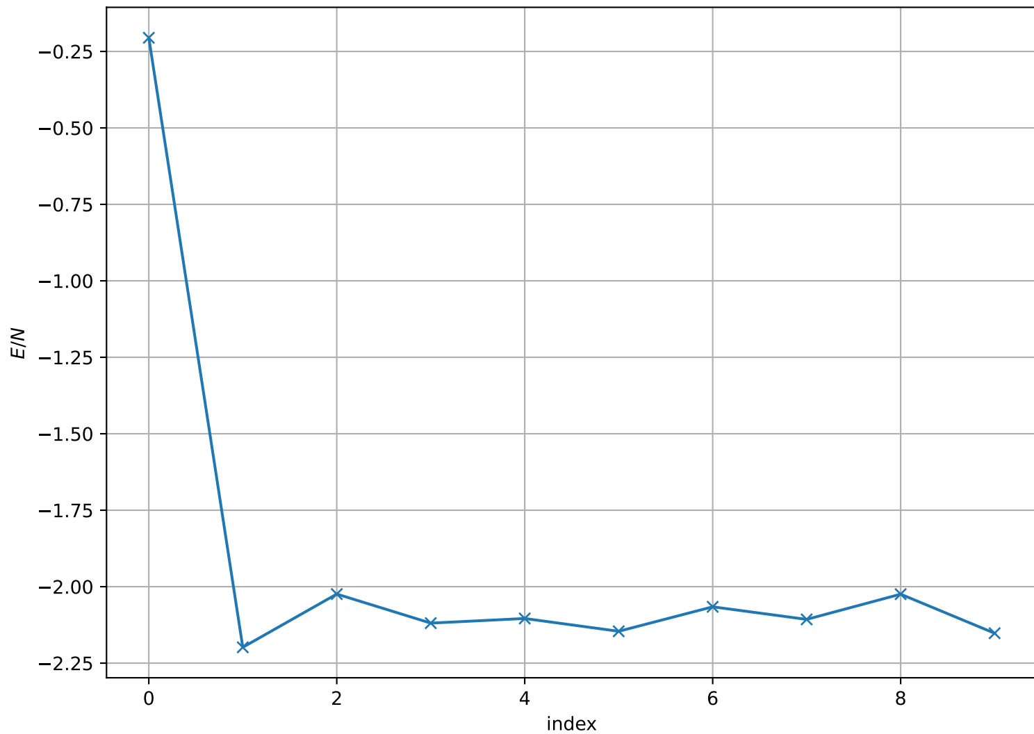
Energy per Site at T = 1.100e + 00 , L = 16
