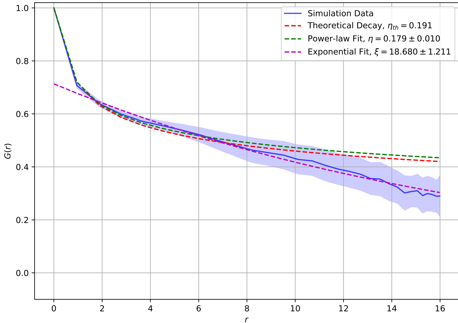
Correlation Function at T = 1.20e + 00 , L = 16
