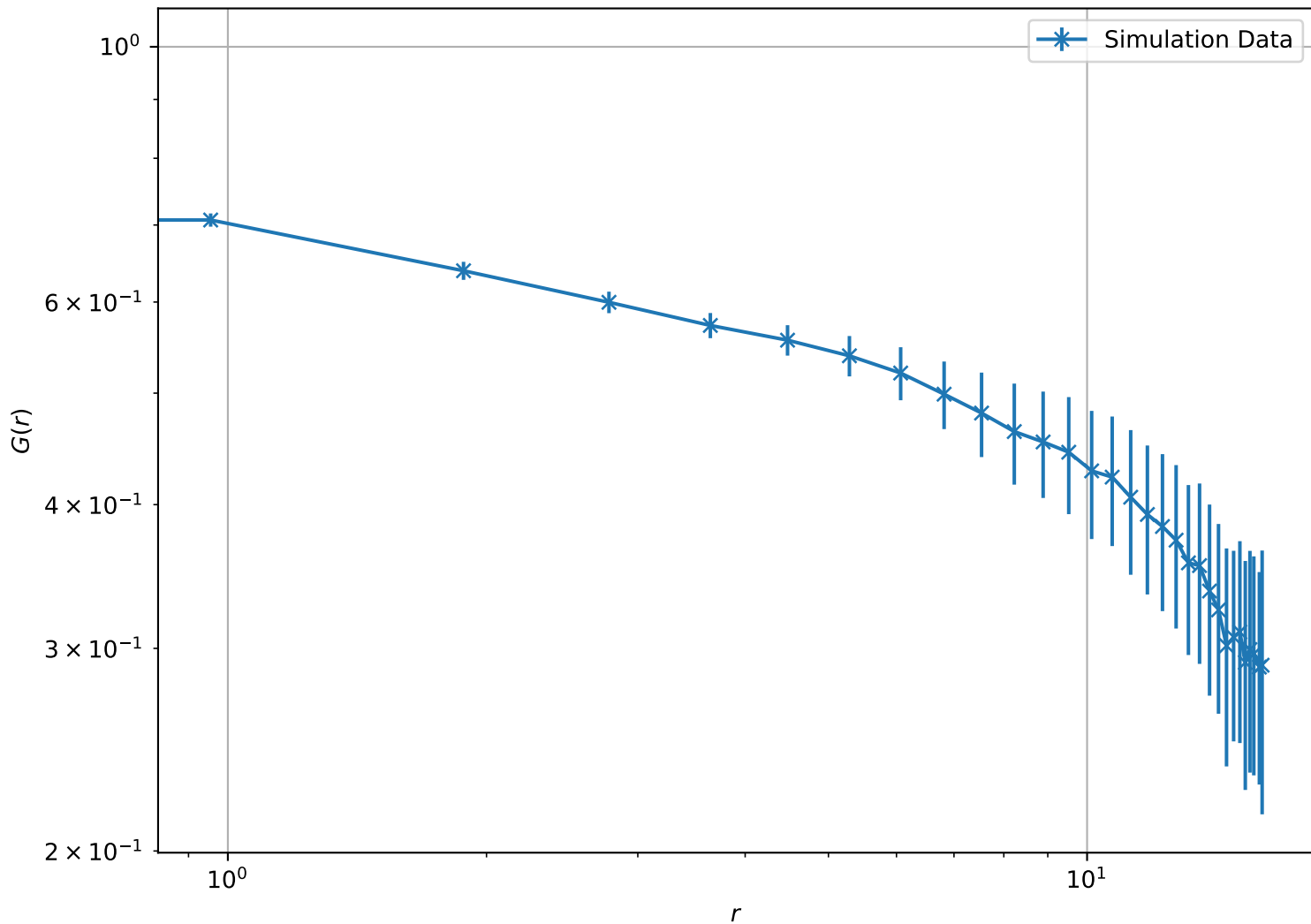
Correlation Function at T = 1.20e + 00 , L = 16 (Log-Log Scale)
