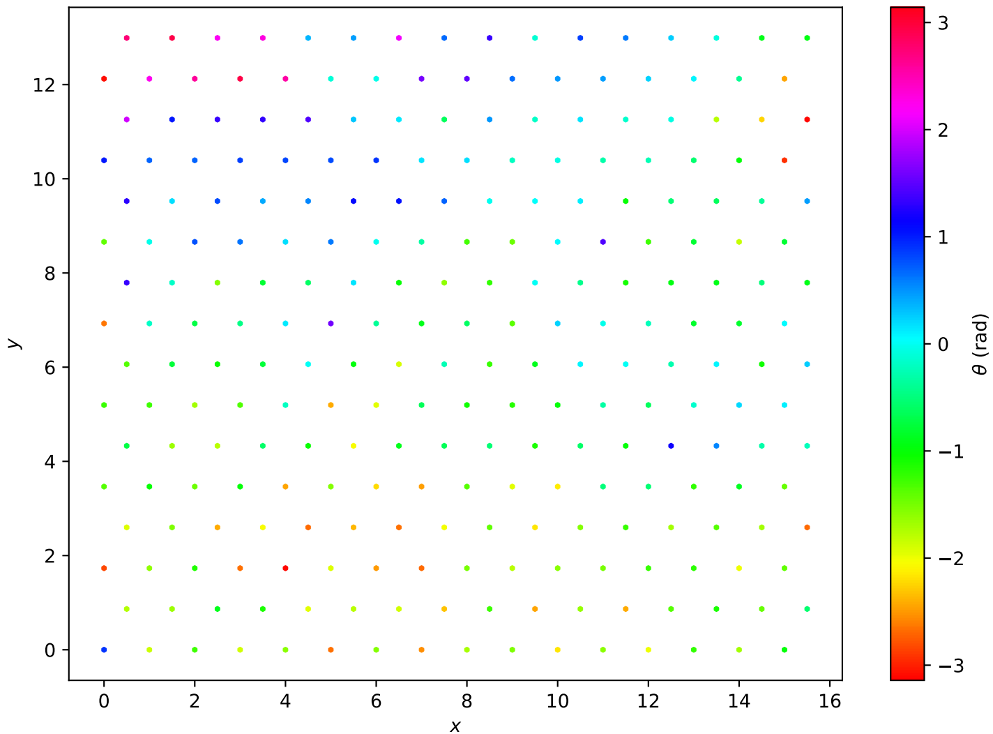
Hexagonal Lattice L=16, T = 1.20e + 00
