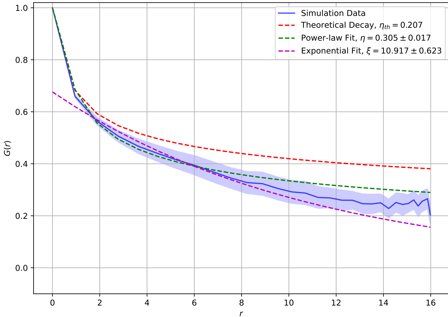
Correlation Function at T = 1.30e + 00 , L = 16
