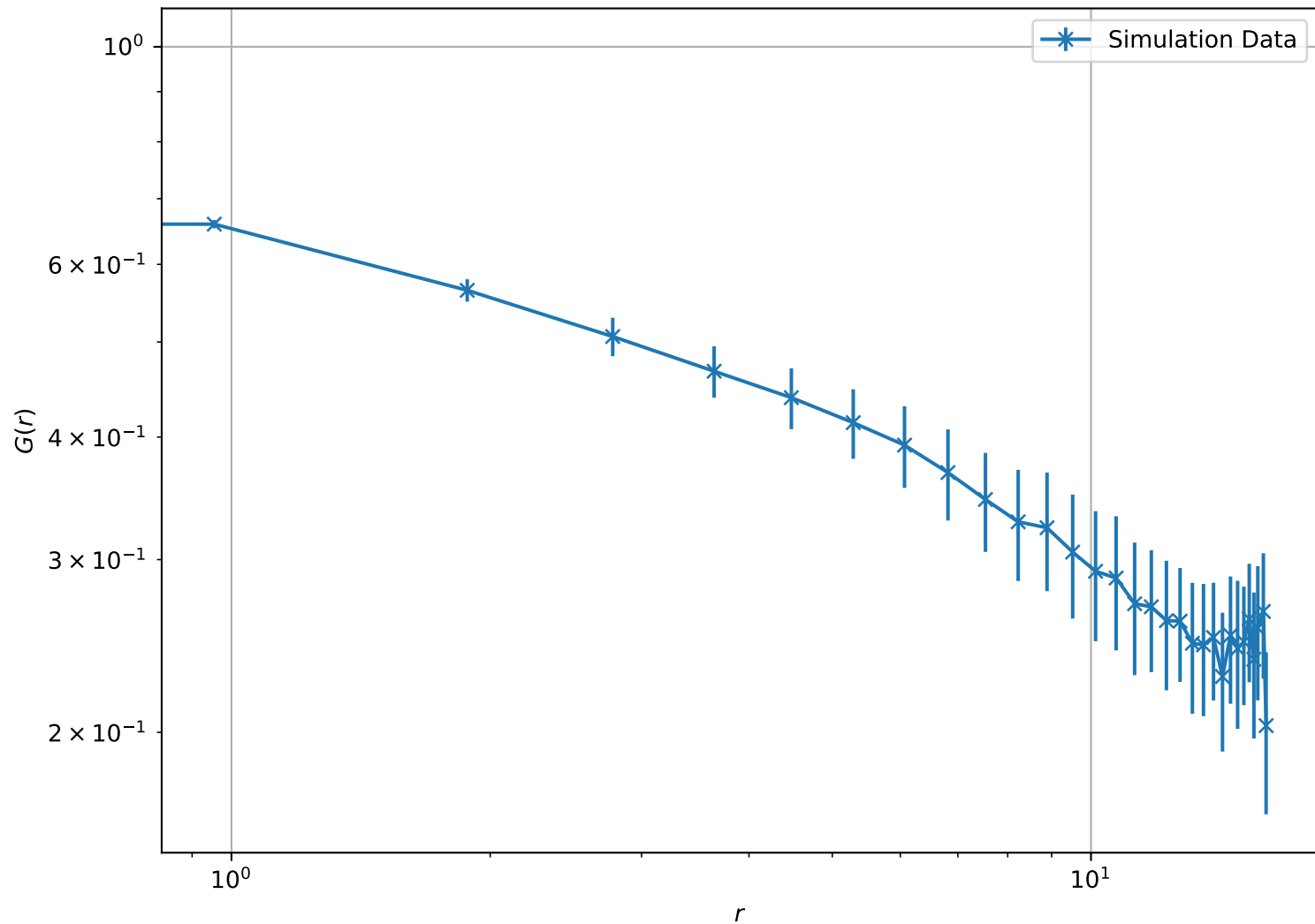
Correlation Function at T = 1.30e + 00 , L = 16 (Log-Log Scale)
