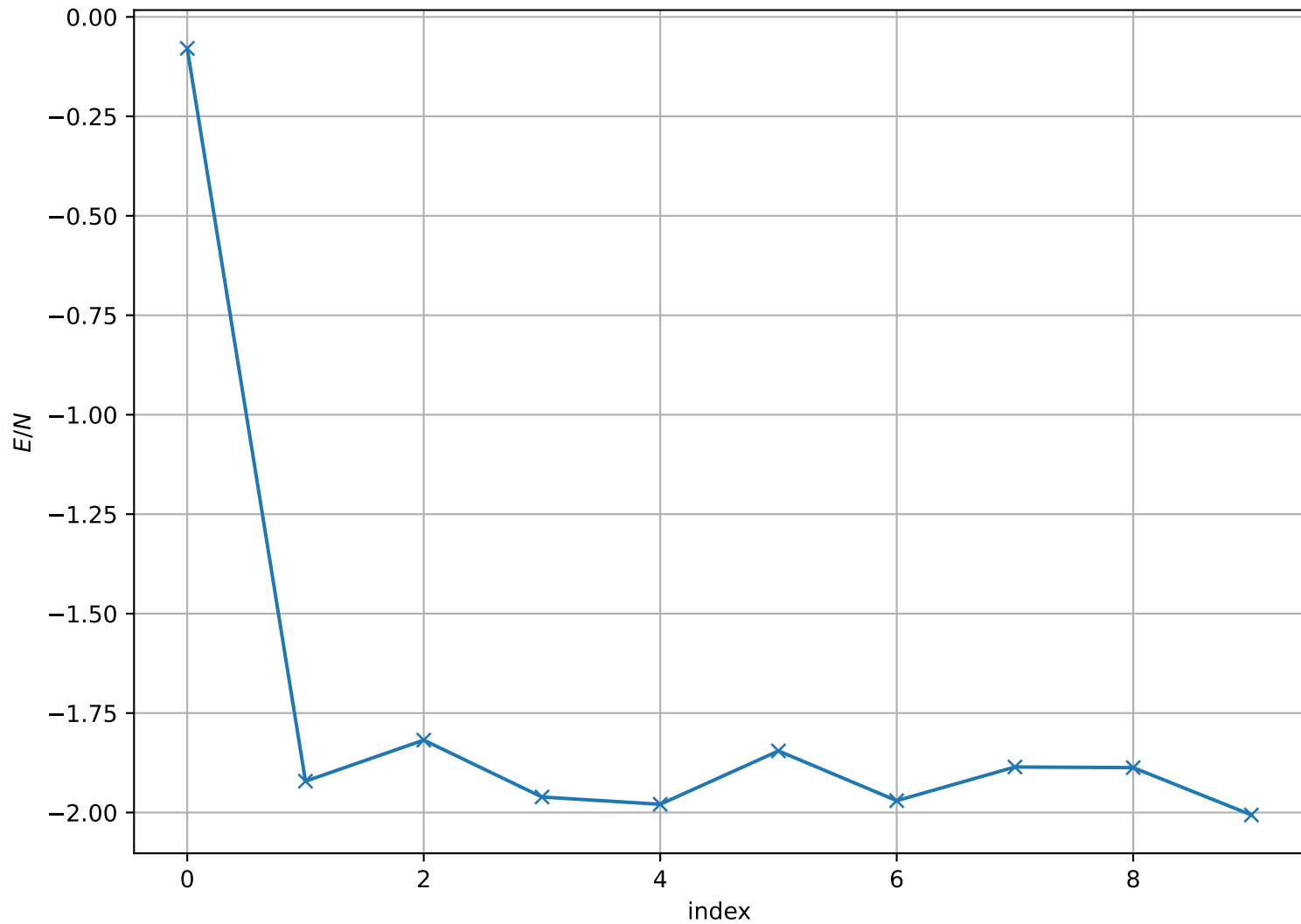
Energy per Site at T = 1.300e + 00 , L = 16
