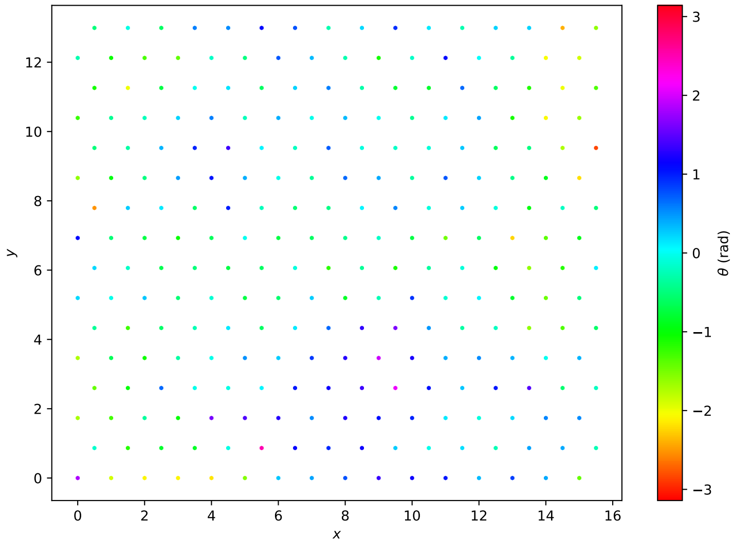
Hexagonal Lattice L=16 , T = 1.30e + 00
