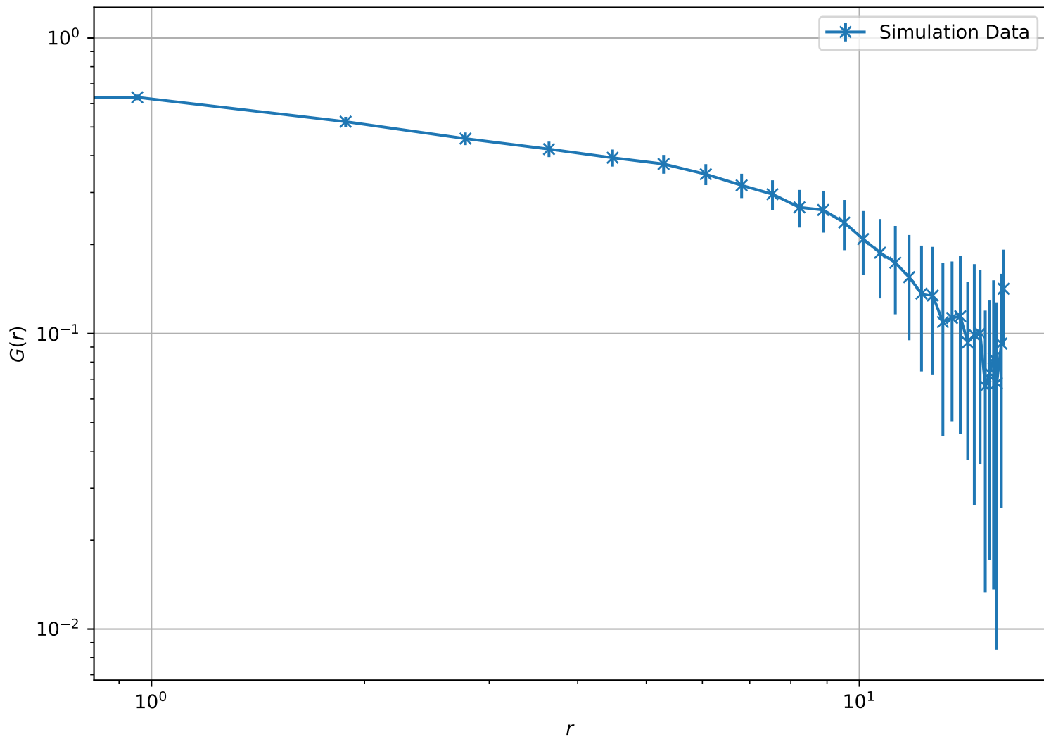
Correlation Function at T = 1.40e + 00 , L = 16 (Log-Log Scale)
