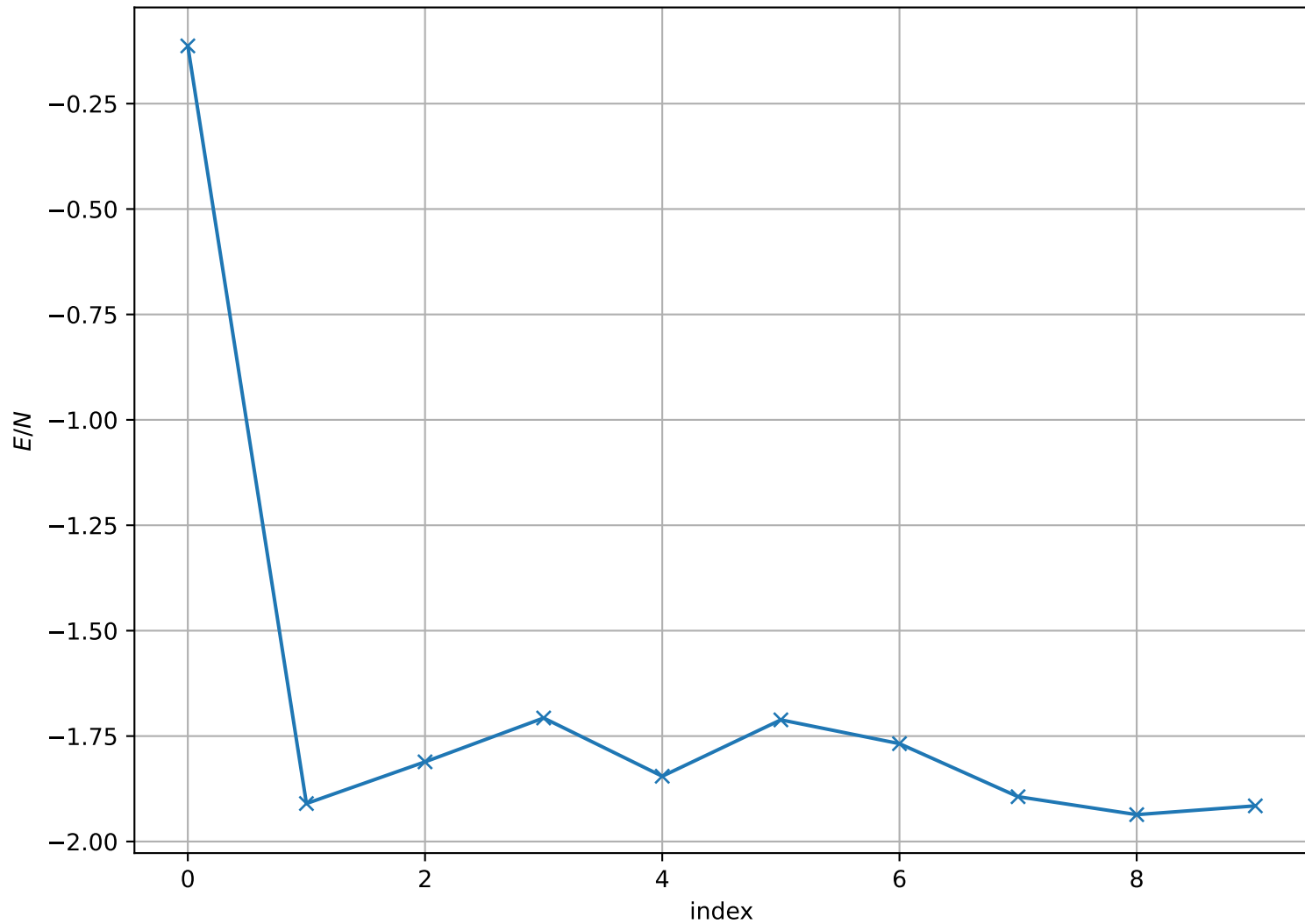
Energy per Site at T = 1.400e + 00 , L = 16
