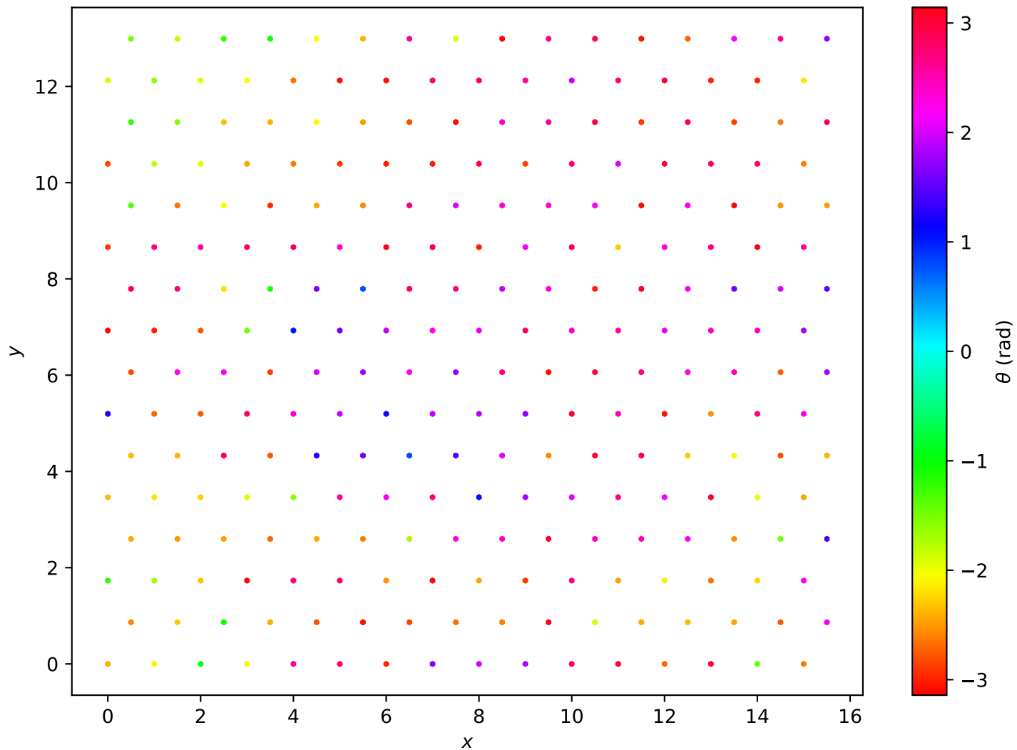
Hexagonal Lattice L=16 , T = 1.40e + 00
