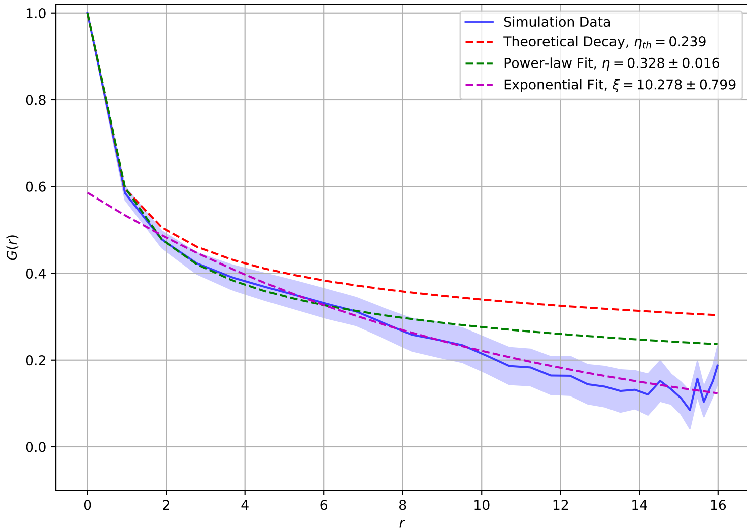
Correlation Function at T = 1.50e + 00 , L = 16
