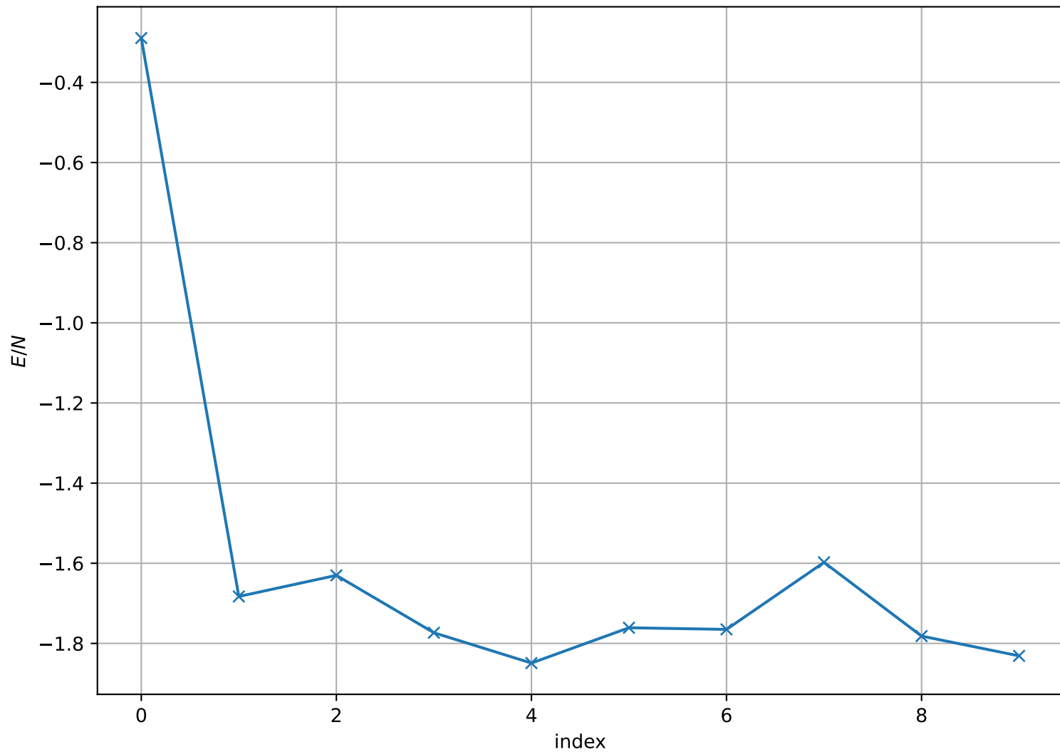
Energy per Site at T = 1.500e + 00 , L = 16
