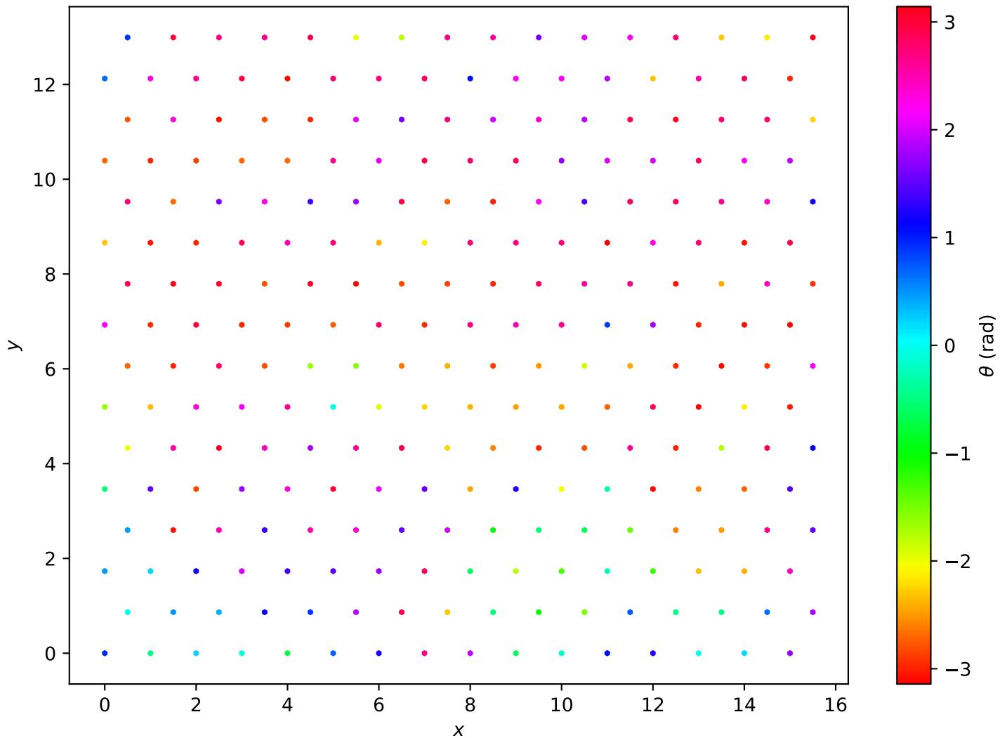
Hexagonal Lattice L=16 , T = 1.50e + 00
