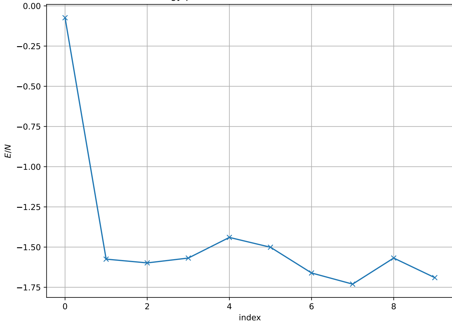
Energy per Site at T = 1.600e + 00 , L = 16
