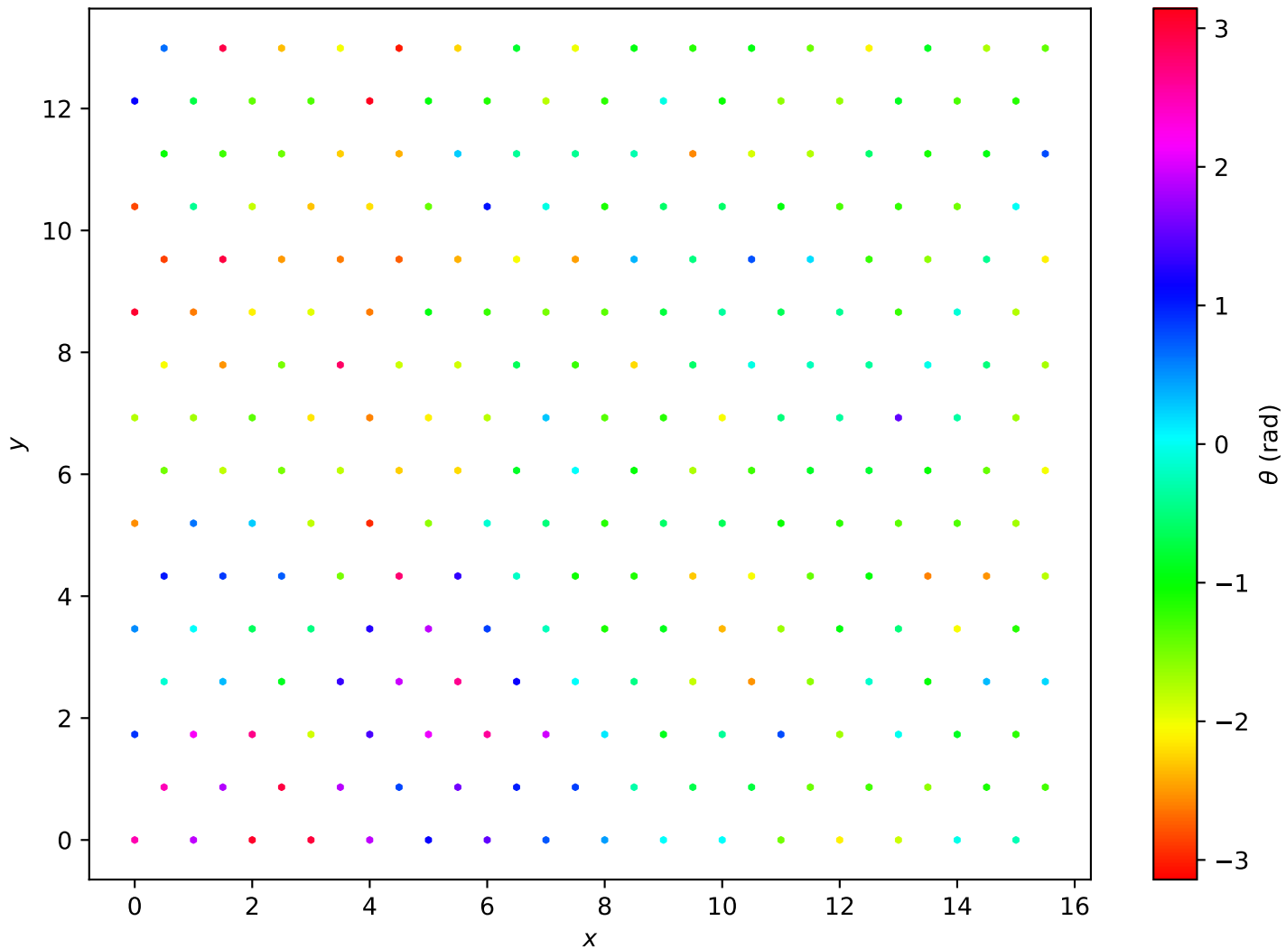
Hexagonal Lattice L=16 , T = 1.60e + 00
