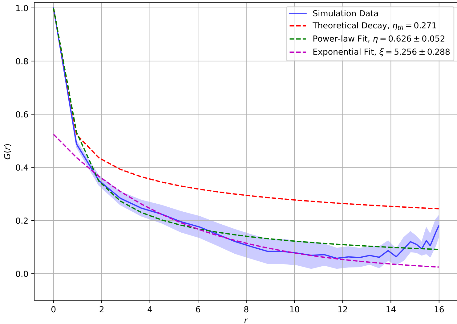
Correlation Function at T = 1.70e + 00 , L = 16
