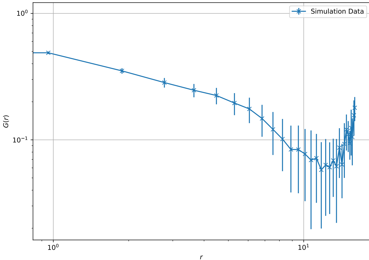
Correlation Function at T = 1.70e + 00 , L = 16 (Log-Log Scale)
