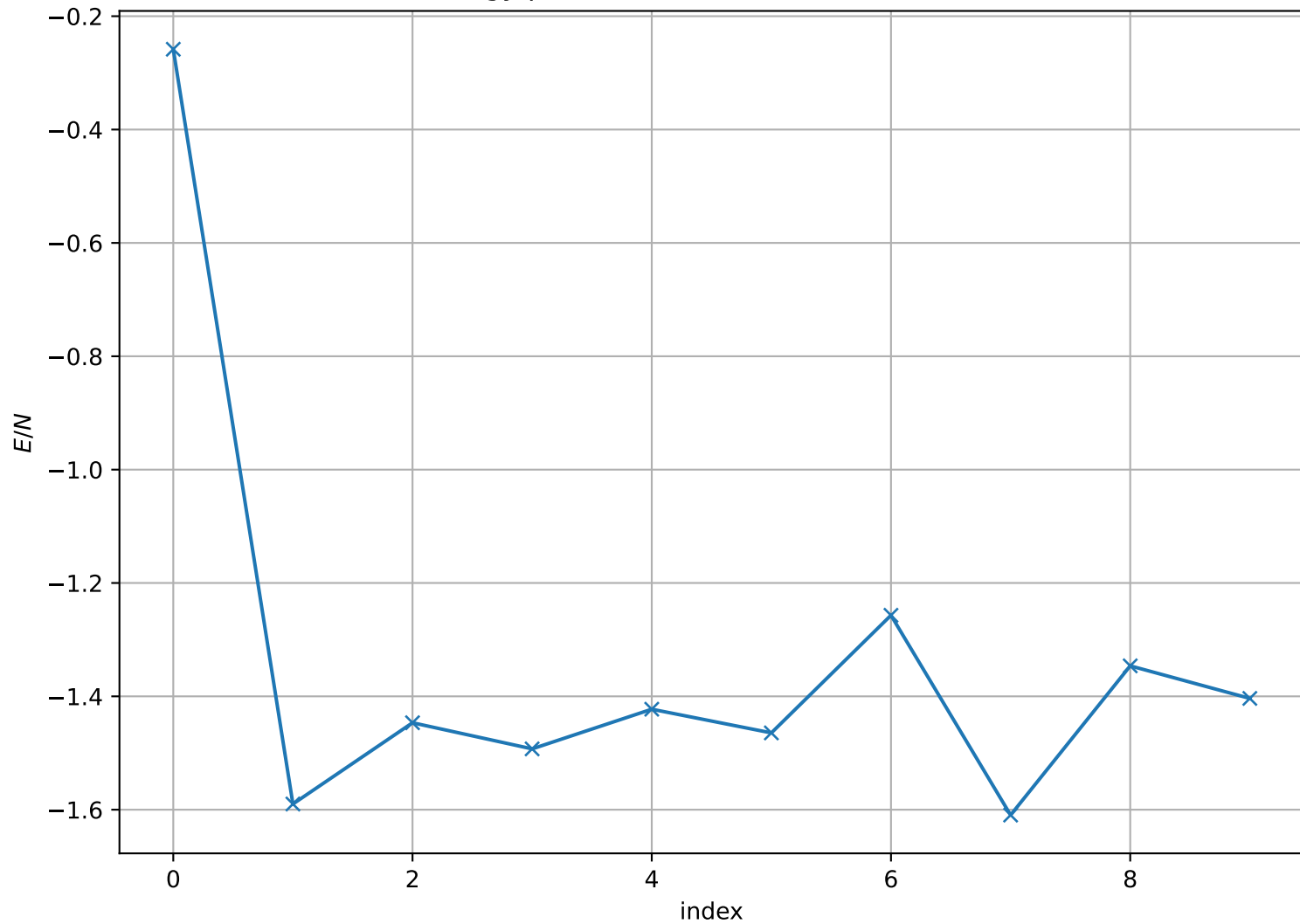
Energy per Site at T = 1.700e + 00 , L = 16
