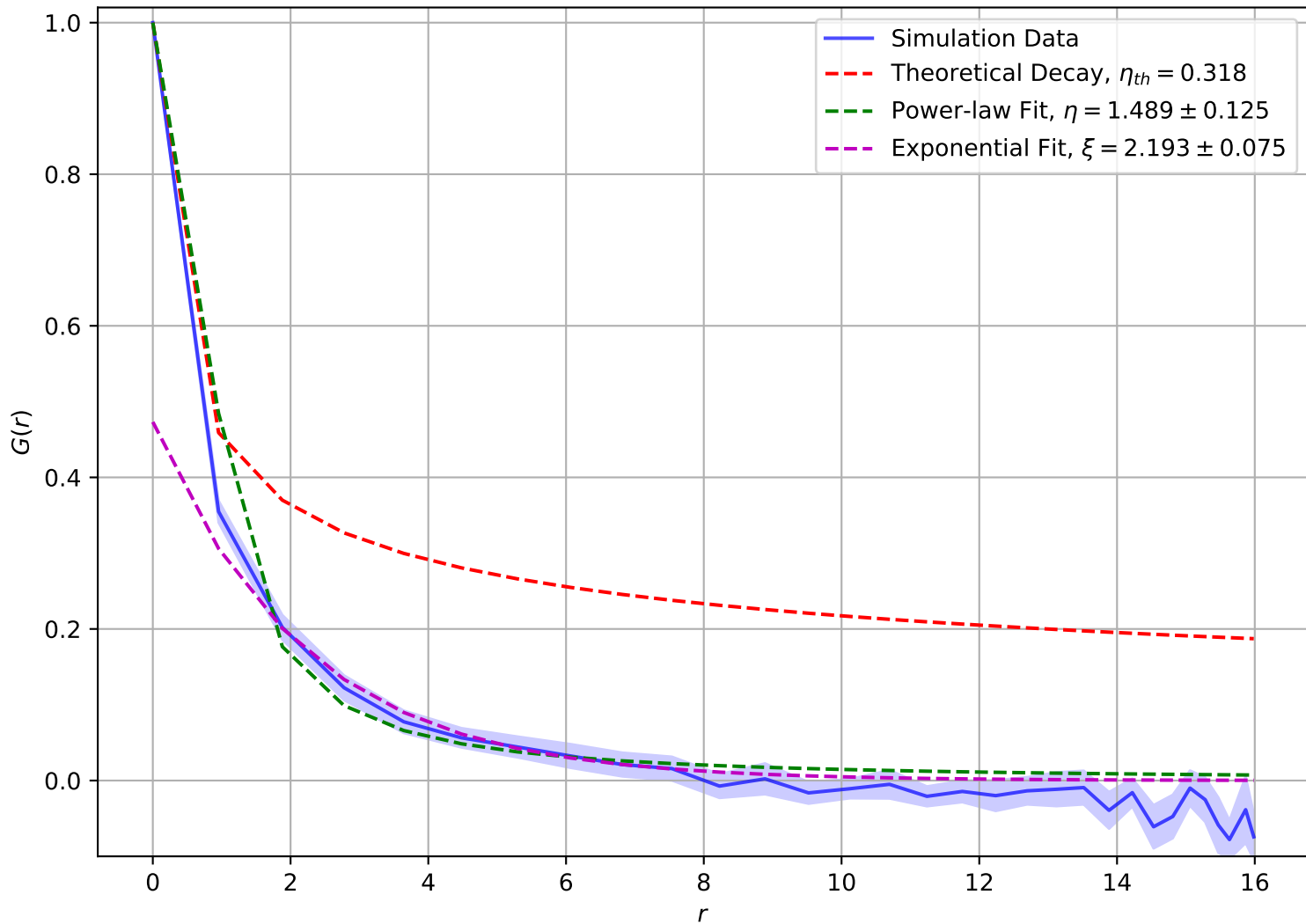
Correlation Function at T = 2.00e + 00 , L = 16
