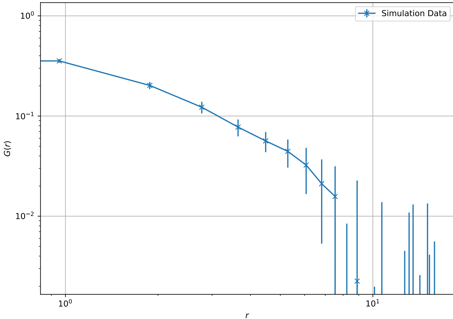
Correlation Function at T = 2.00e + 00 , L = 16 (Log-Log Scale)
