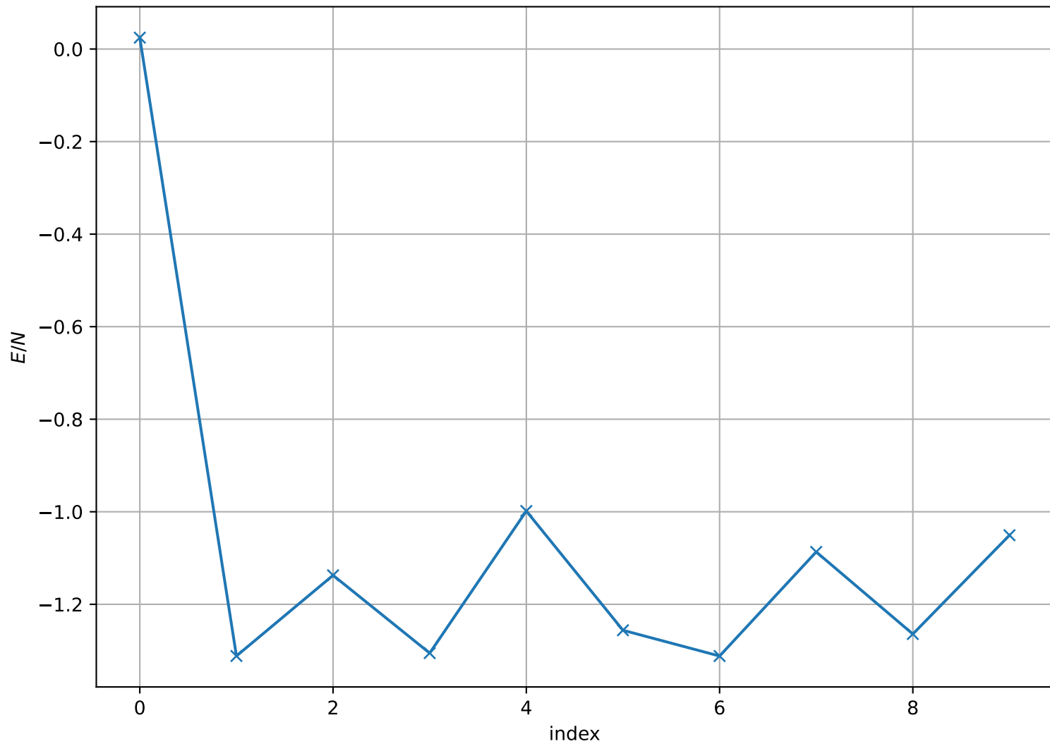
Energy per Site at T = 2.000e + 00 , L = 16
