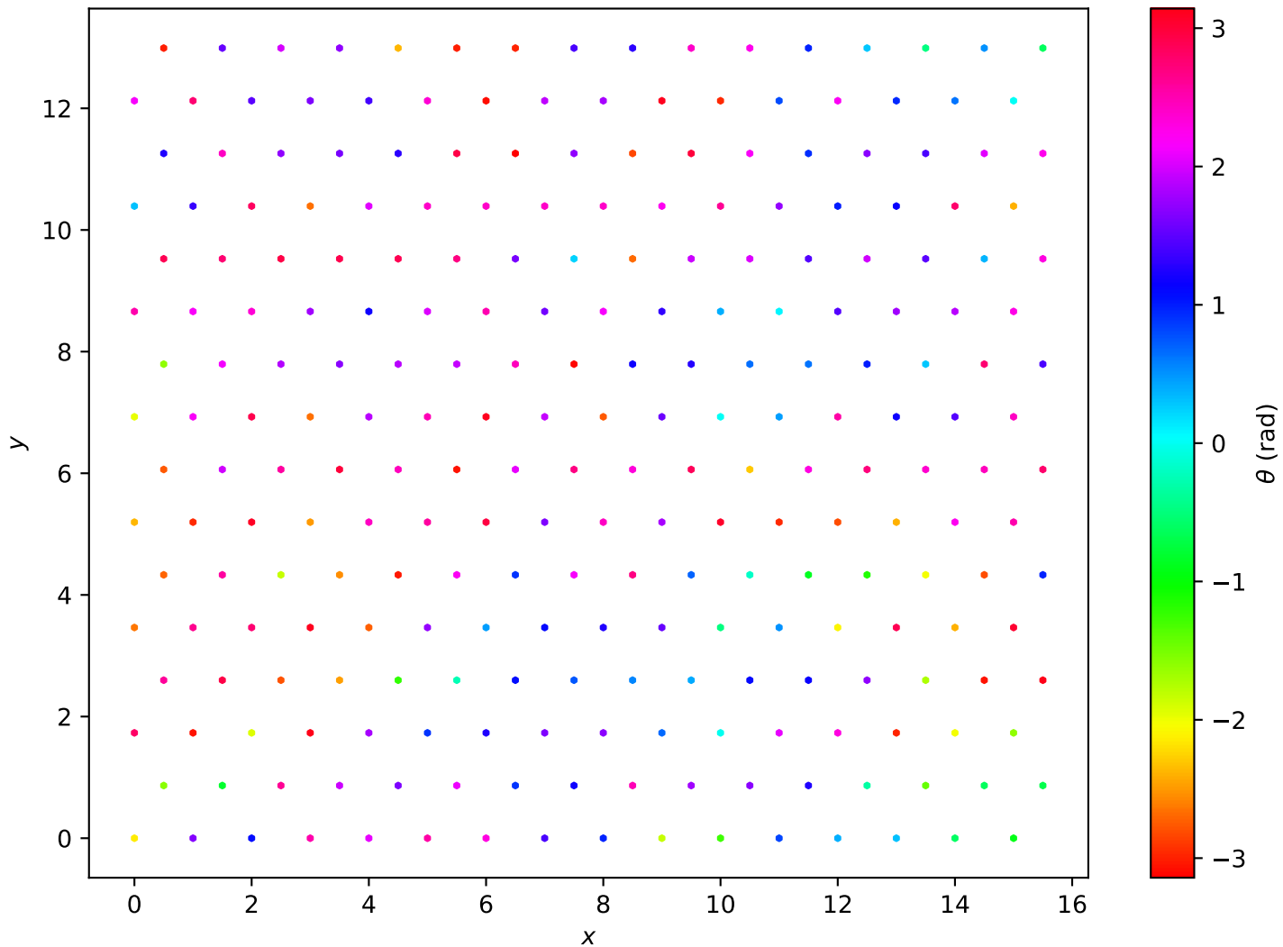
Hexagonal Lattice L=16 , T = 2.00e + 00
