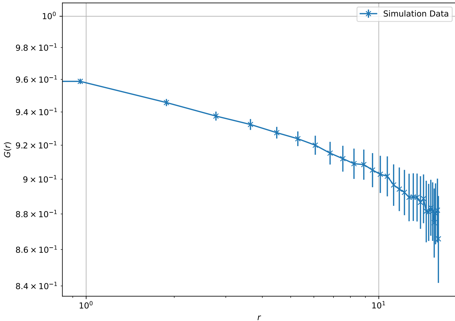
Correlation Function at T = 2.00e - 01 , L = 16 (Log-Log Scale)
