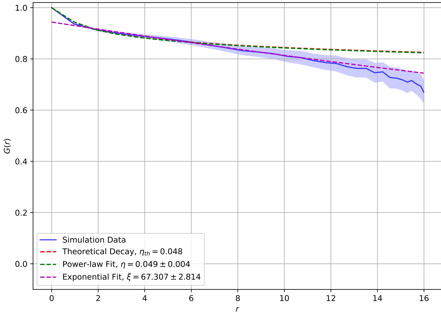
Correlation Function at T = 3.00e - 01 , L = 16
