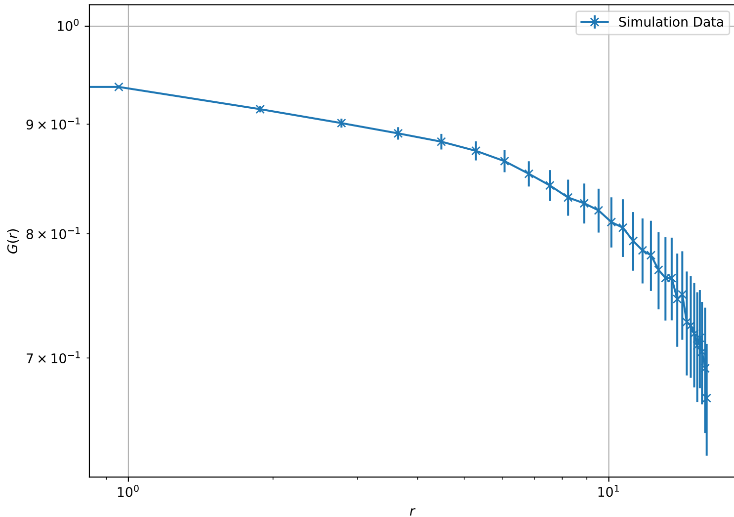
Correlation Function at T = 3.00e - 01 , L = 16 (Log-Log Scale)
