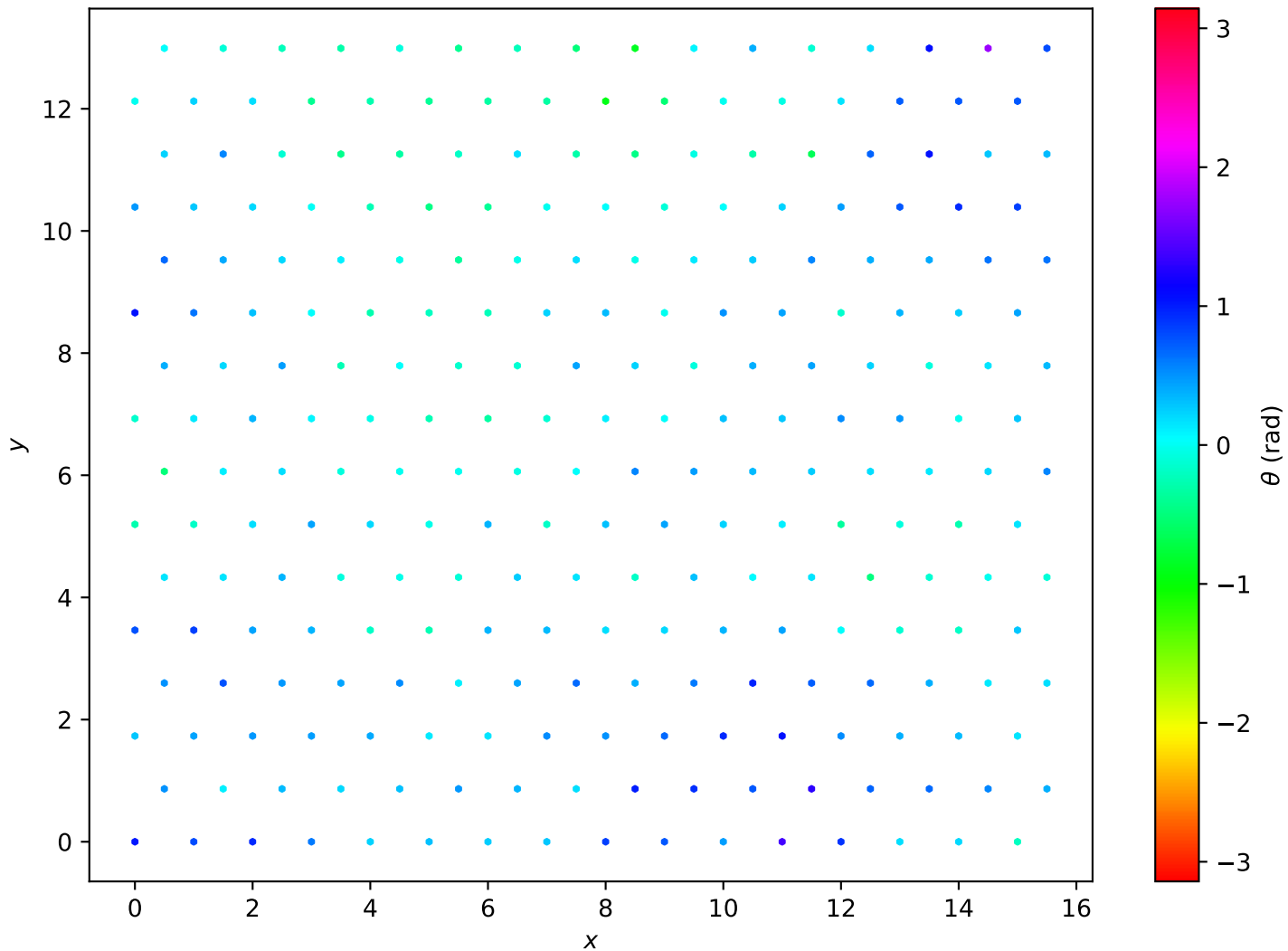
Hexagonal Lattice L=16 , T = 3.00e - 01
