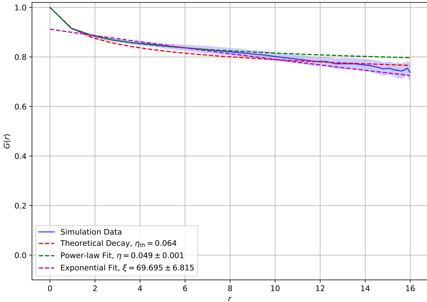
Correlation Function at T = 4.00e - 01 , L = 16
