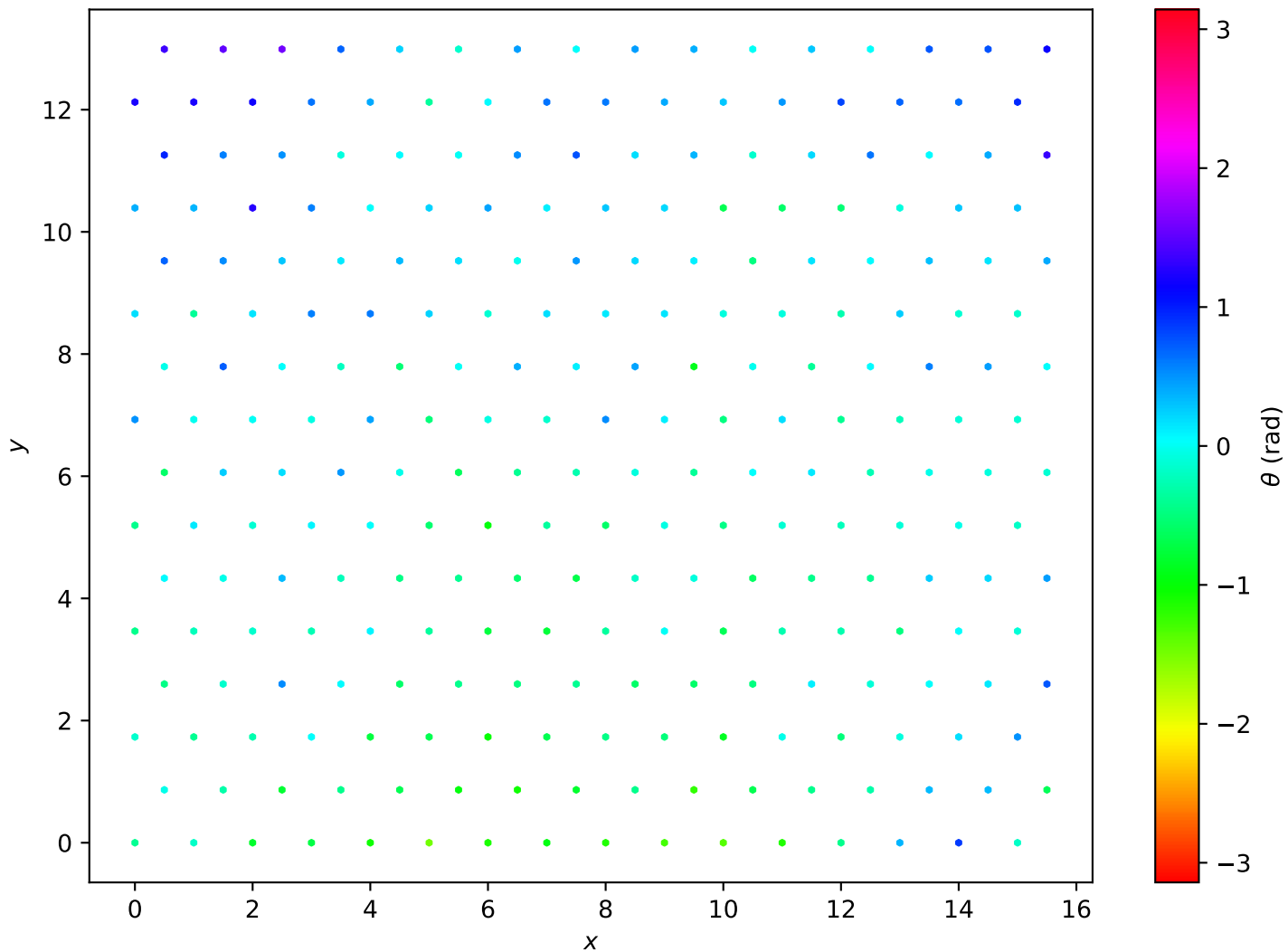
Hexagonal Lattice L=16 , T = 4.00e - 01
