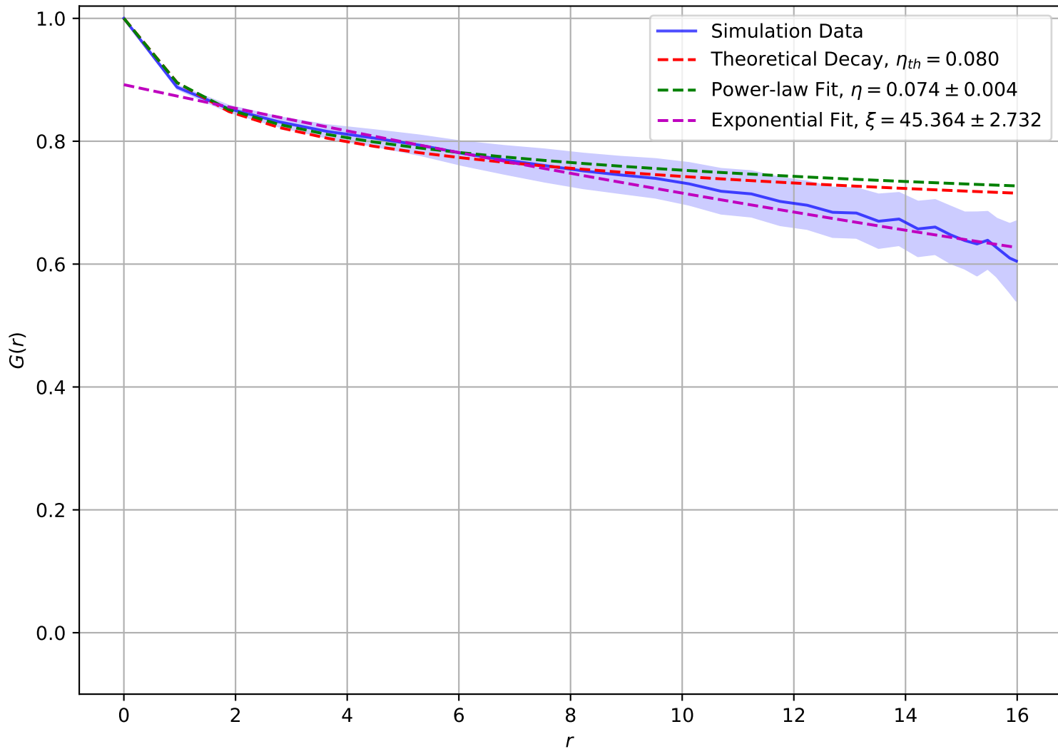
Correlation Function at T = 5.00e - 01 , L = 16
