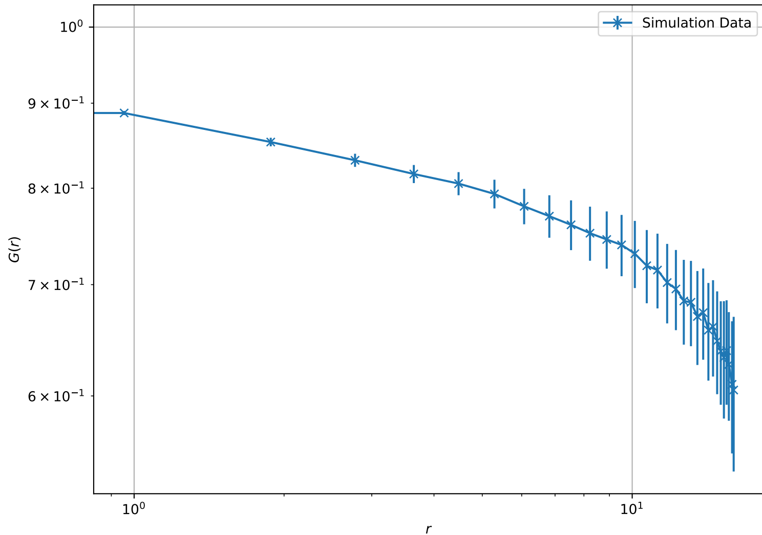
Correlation Function at T = 5.00e - 01 , L = 16 (Log-Log Scale)
