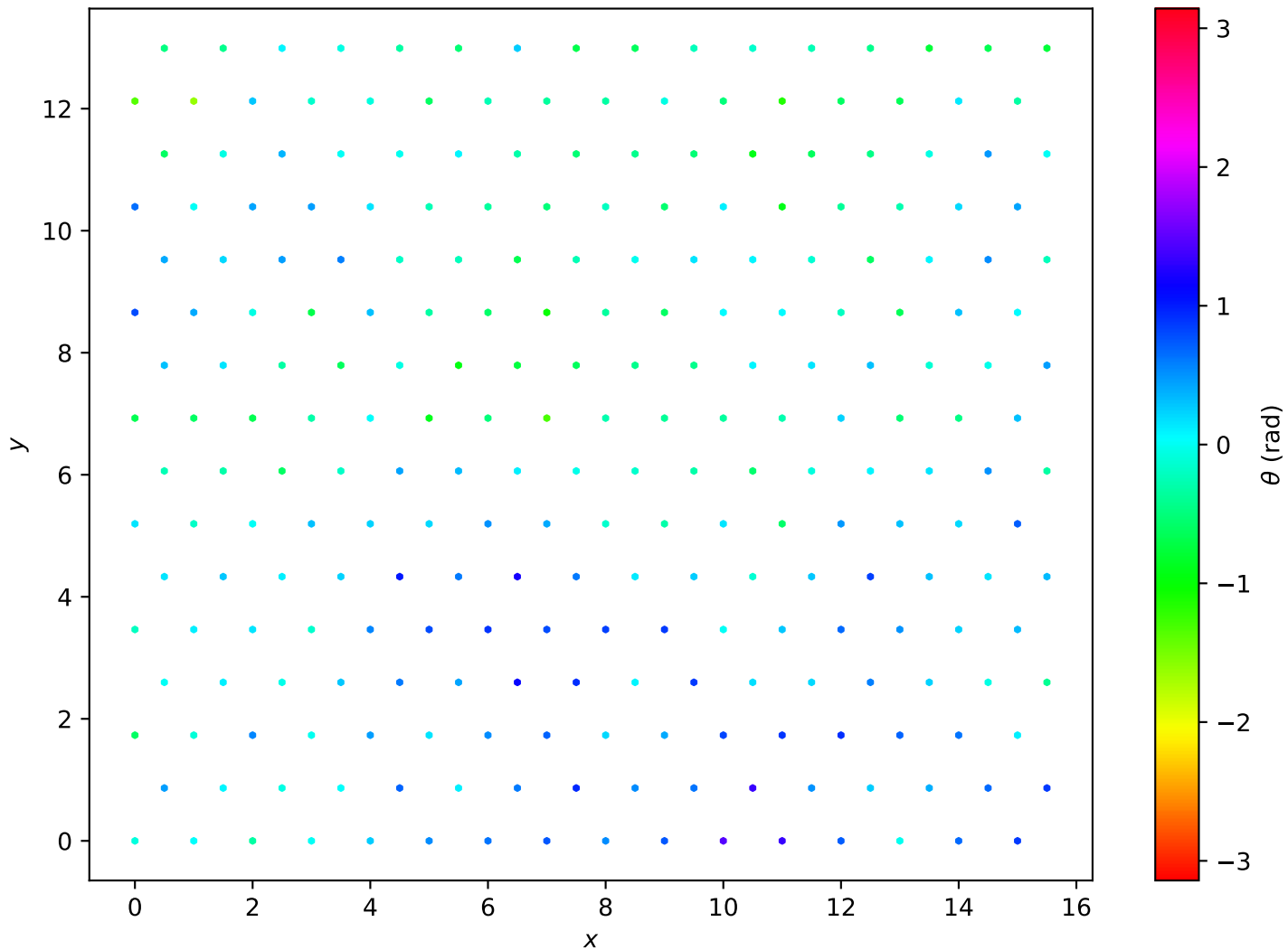
Hexagonal Lattice L=16 , T = 5.00e - 01
