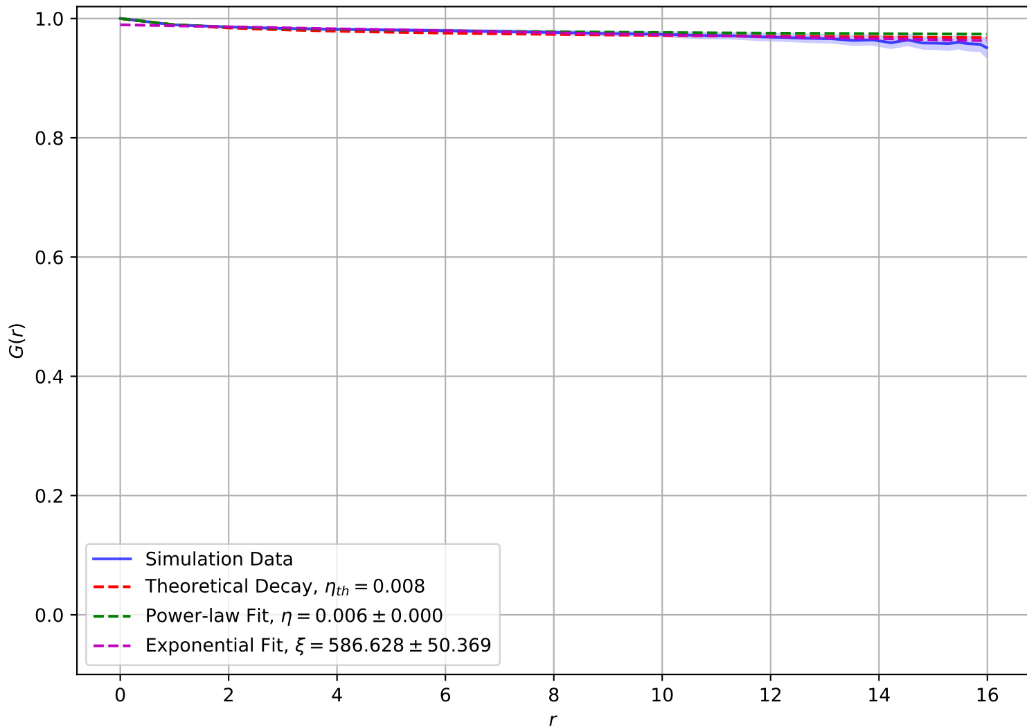
Correlation Function at T = 5.00\text{e} - 02 , L = 16
