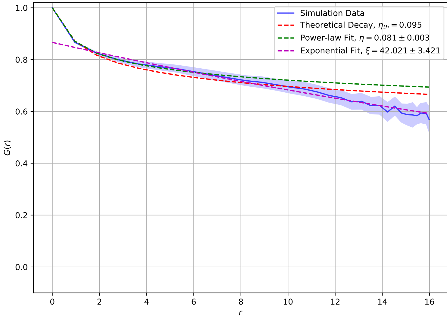
Correlation Function at T = 6.00e - 01 , L = 16
