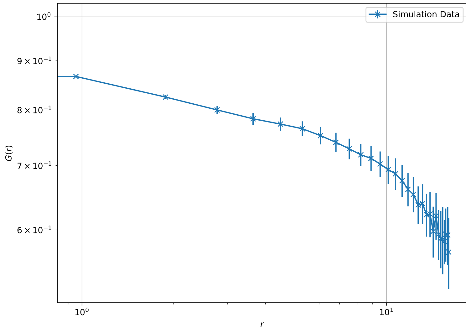
Correlation Function at T = 6.00e - 01 , L = 16 (Log-Log Scale)
