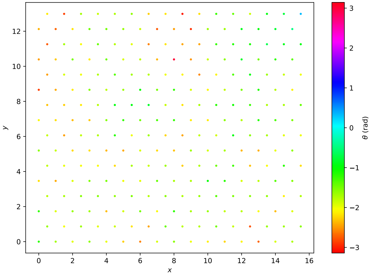
Hexagonal Lattice L=16 , T = 6.00e - 01
