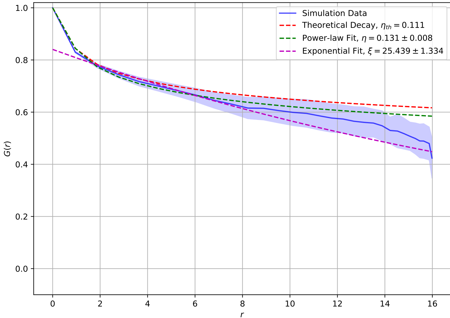
Correlation Function at T = 7.00e - 01 , L = 16
