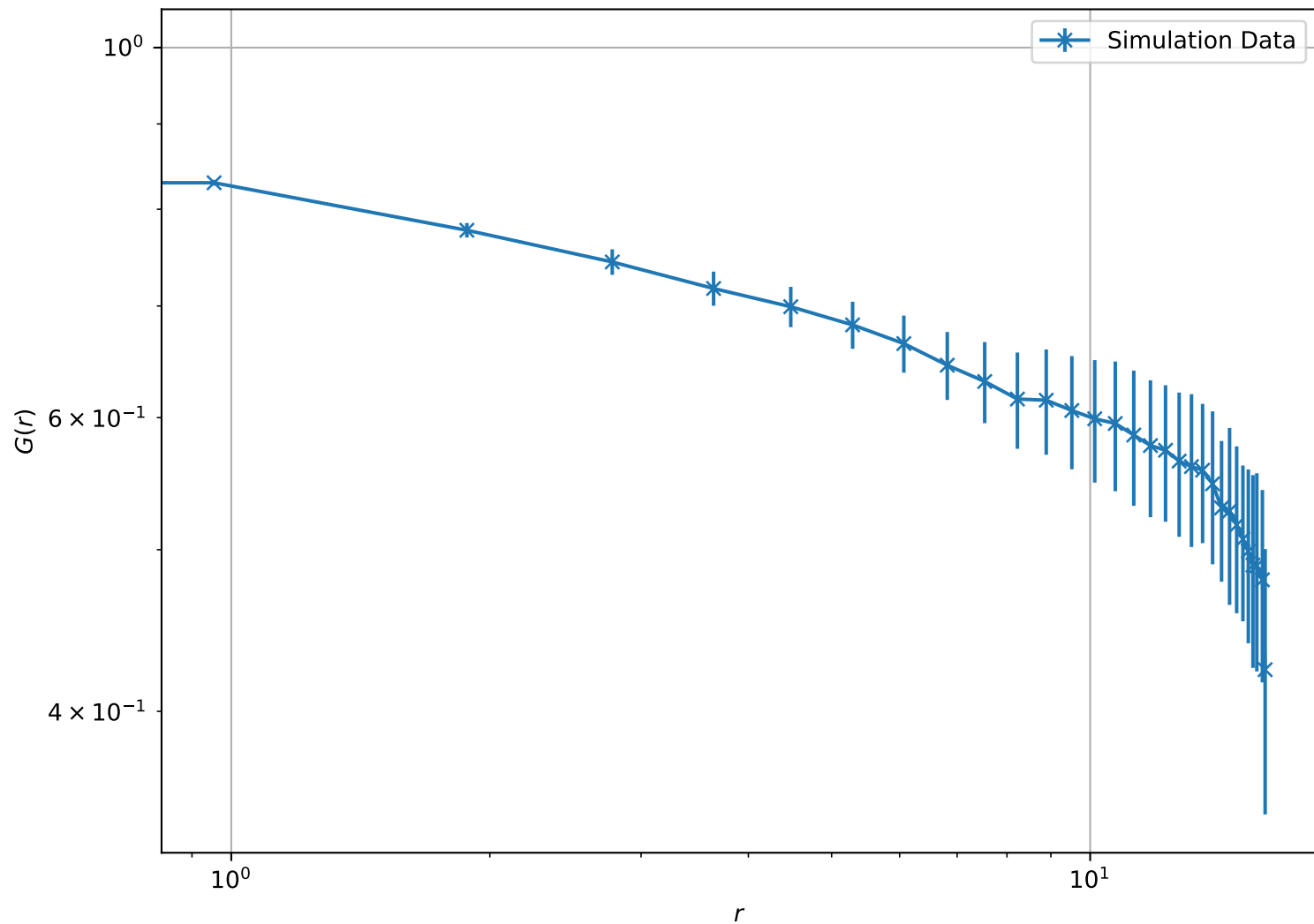
Correlation Function at T = 7.00e - 01 , L = 16 (Log-Log Scale)
