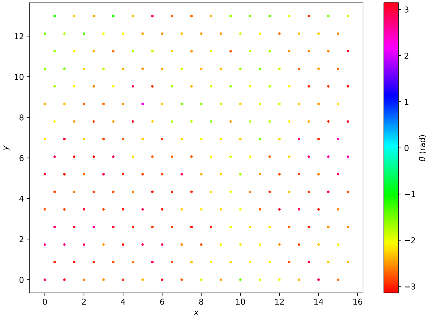
Hexagonal Lattice L=16 , T = 7.00e - 01
