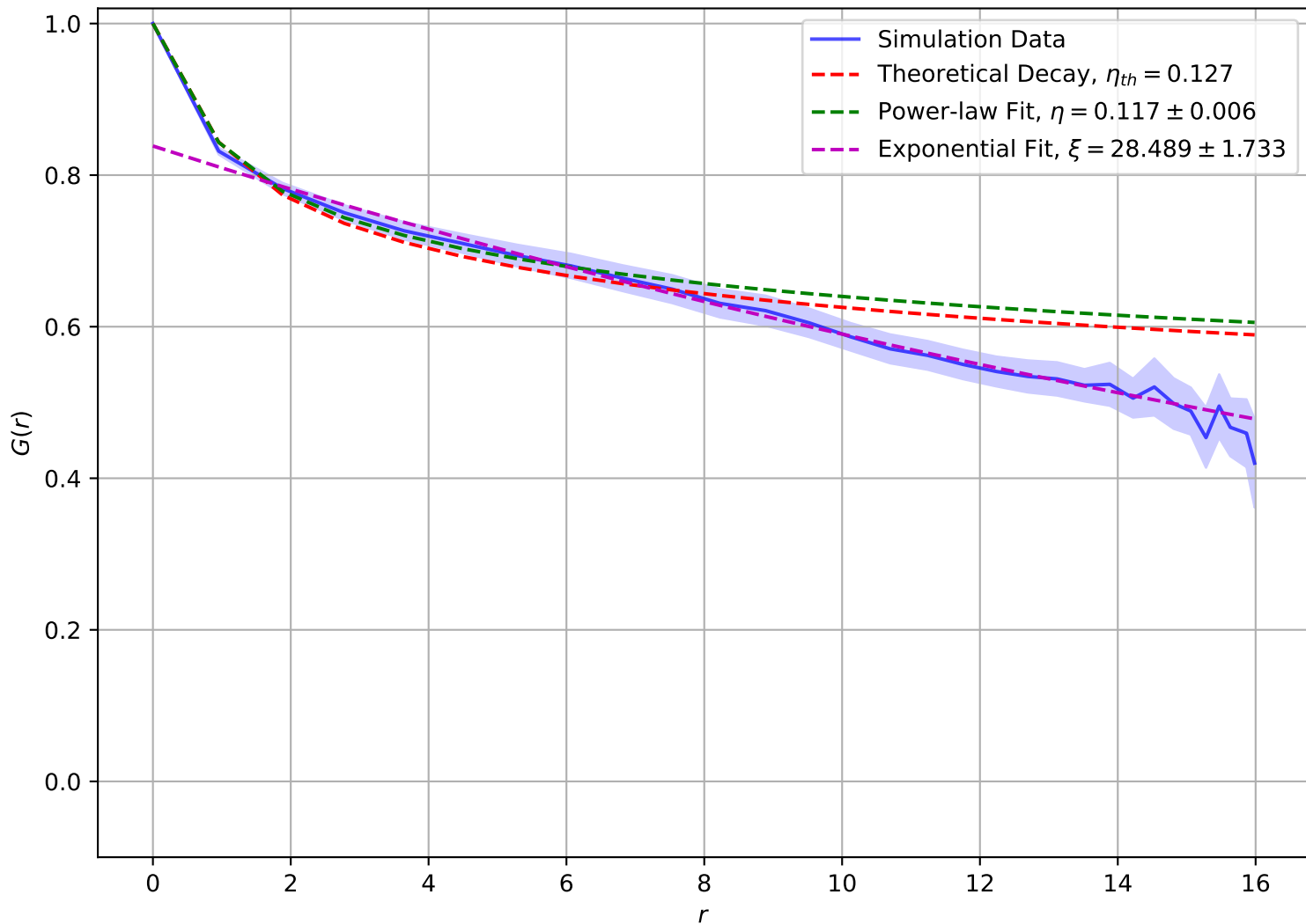
Correlation Function at T = 8.00e - 01 , L = 16
