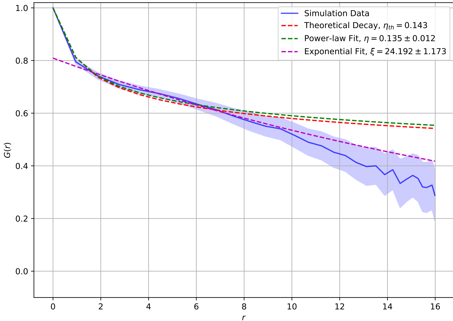
Correlation Function at T = 9.00e - 01 , L = 16
