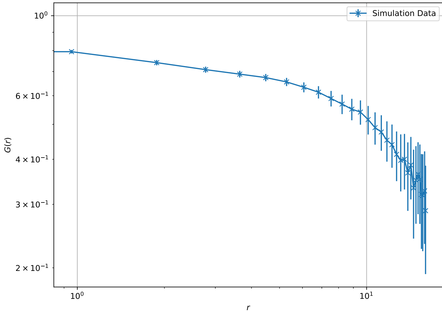
Correlation Function at T = 9.00e - 01 , L = 16 (Log-Log Scale)
