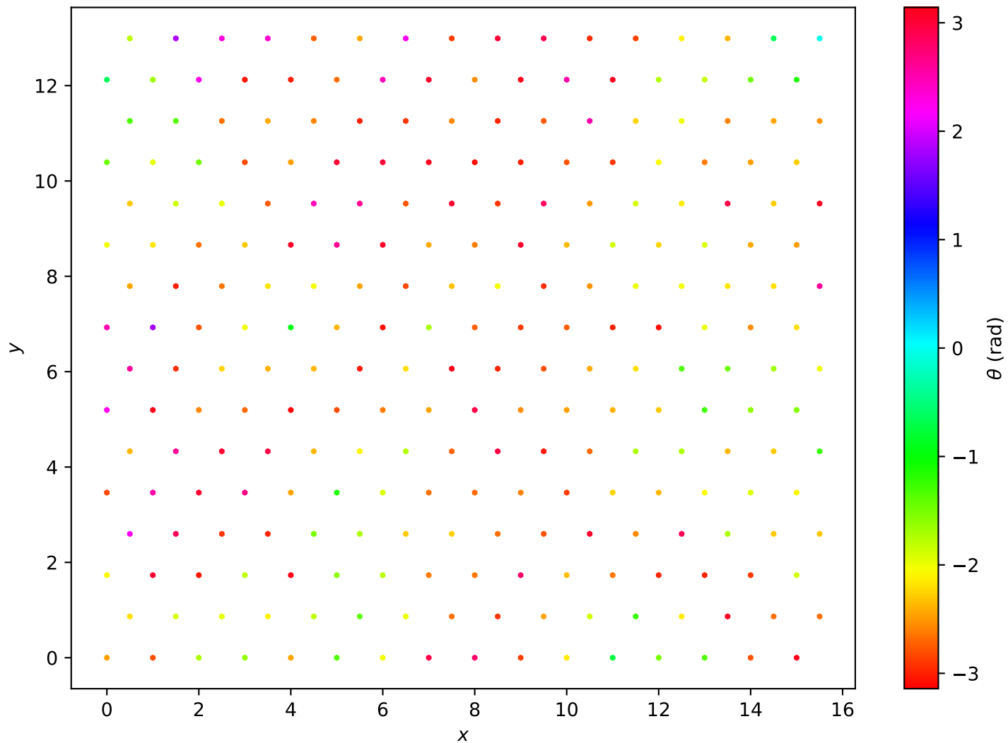
Hexagonal Lattice L=16 , T = 9.00e - 01
