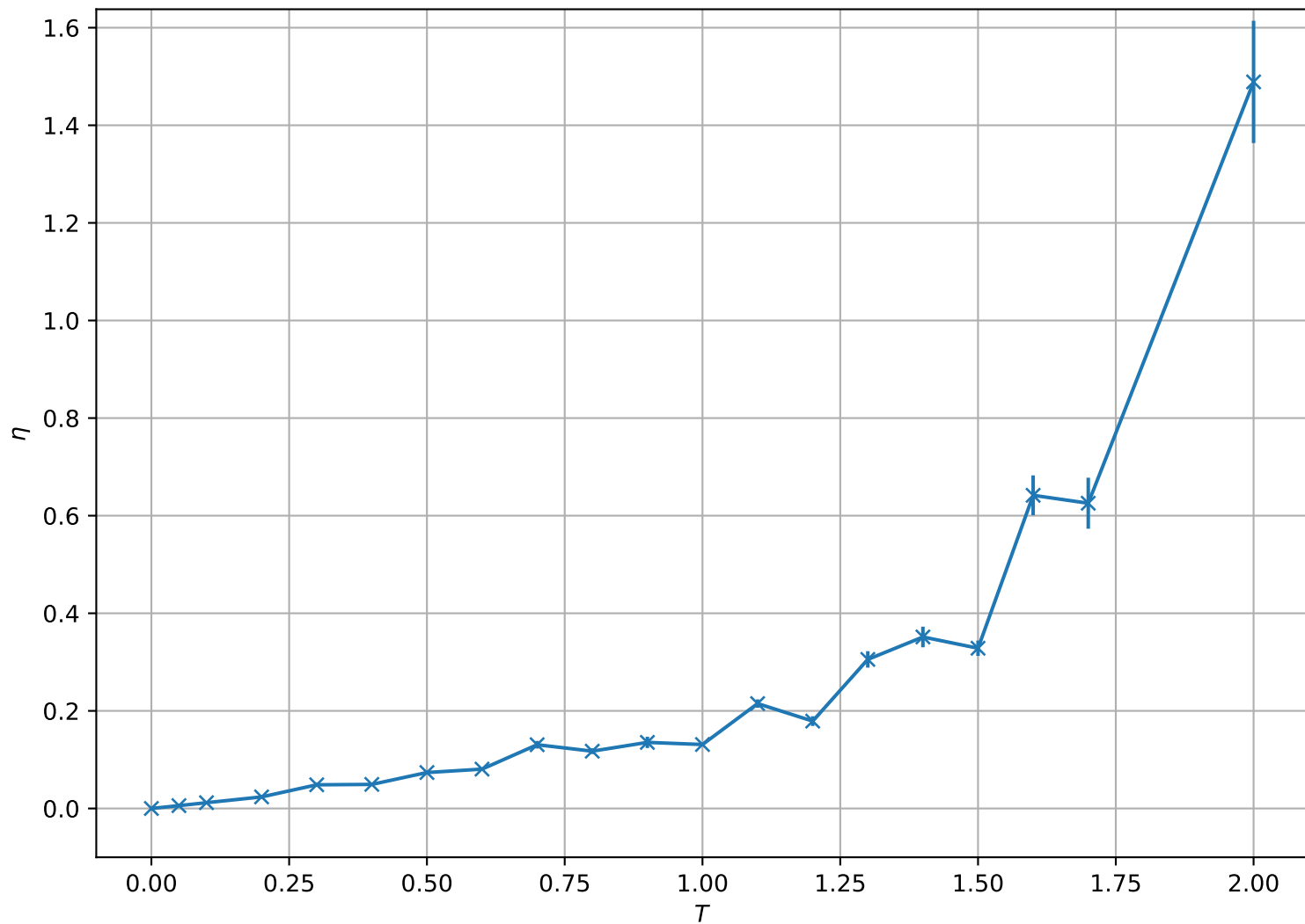
Critical Exponent \eta vs Temperature for L = 16
