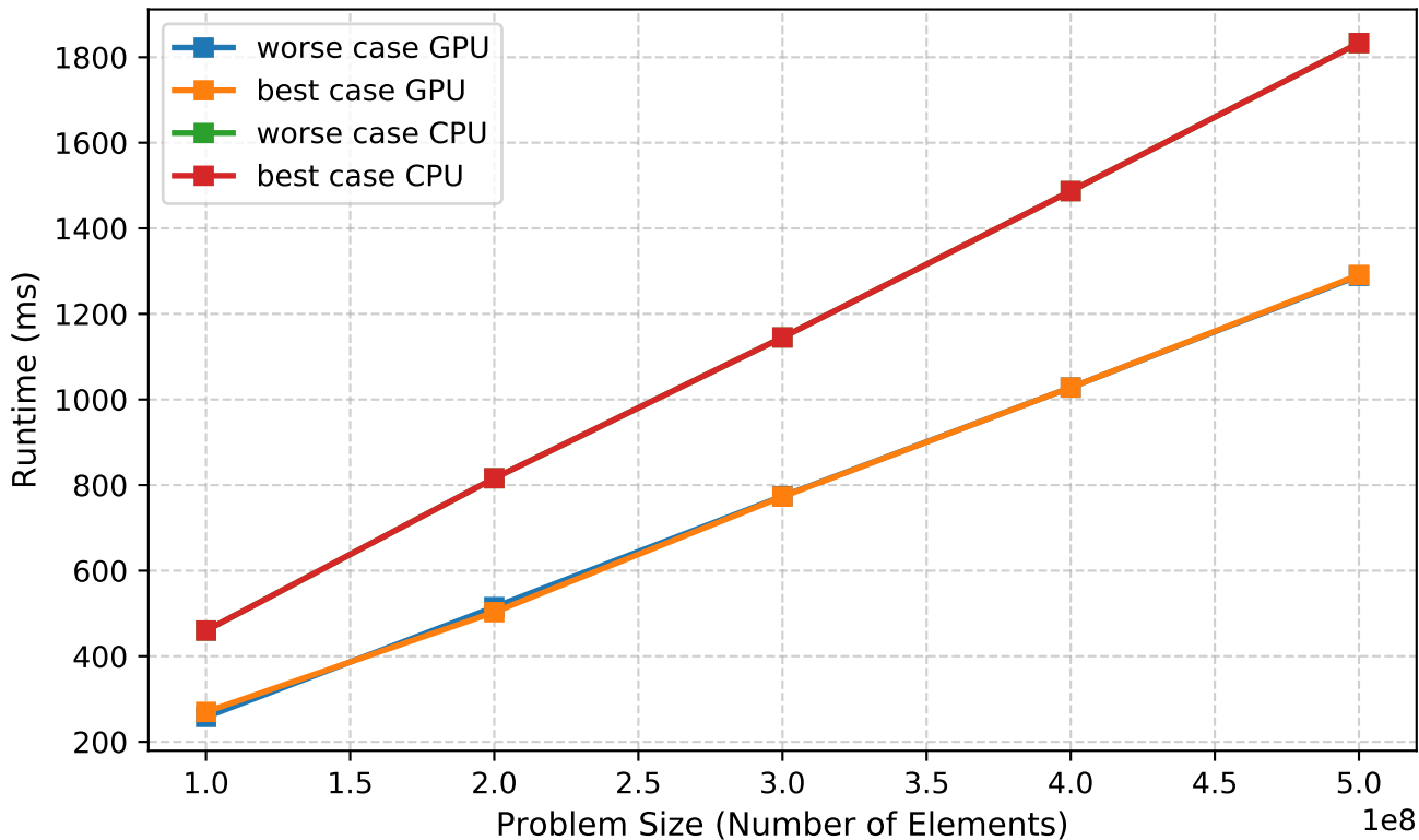
Comparision of sorted vs unsorted array in radix sort
