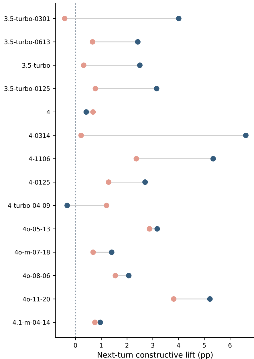
a Adjacent-turn lift after scaffolded support
